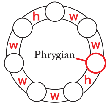
Phrygian Scale
