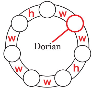
Dorian Scale
